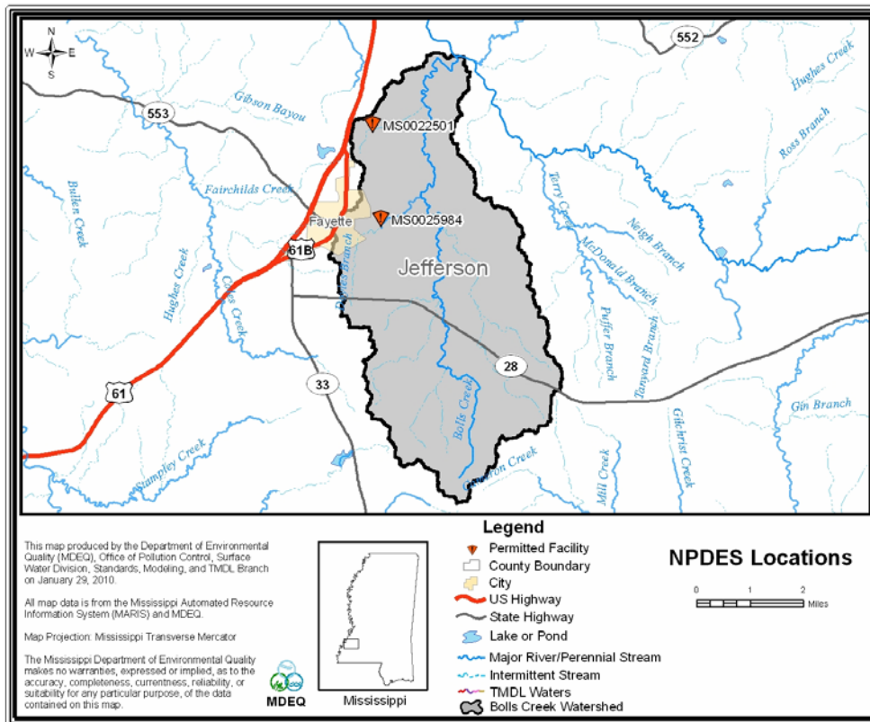
Figure 6. Bolls Creek NPDES Permitted Facilities
