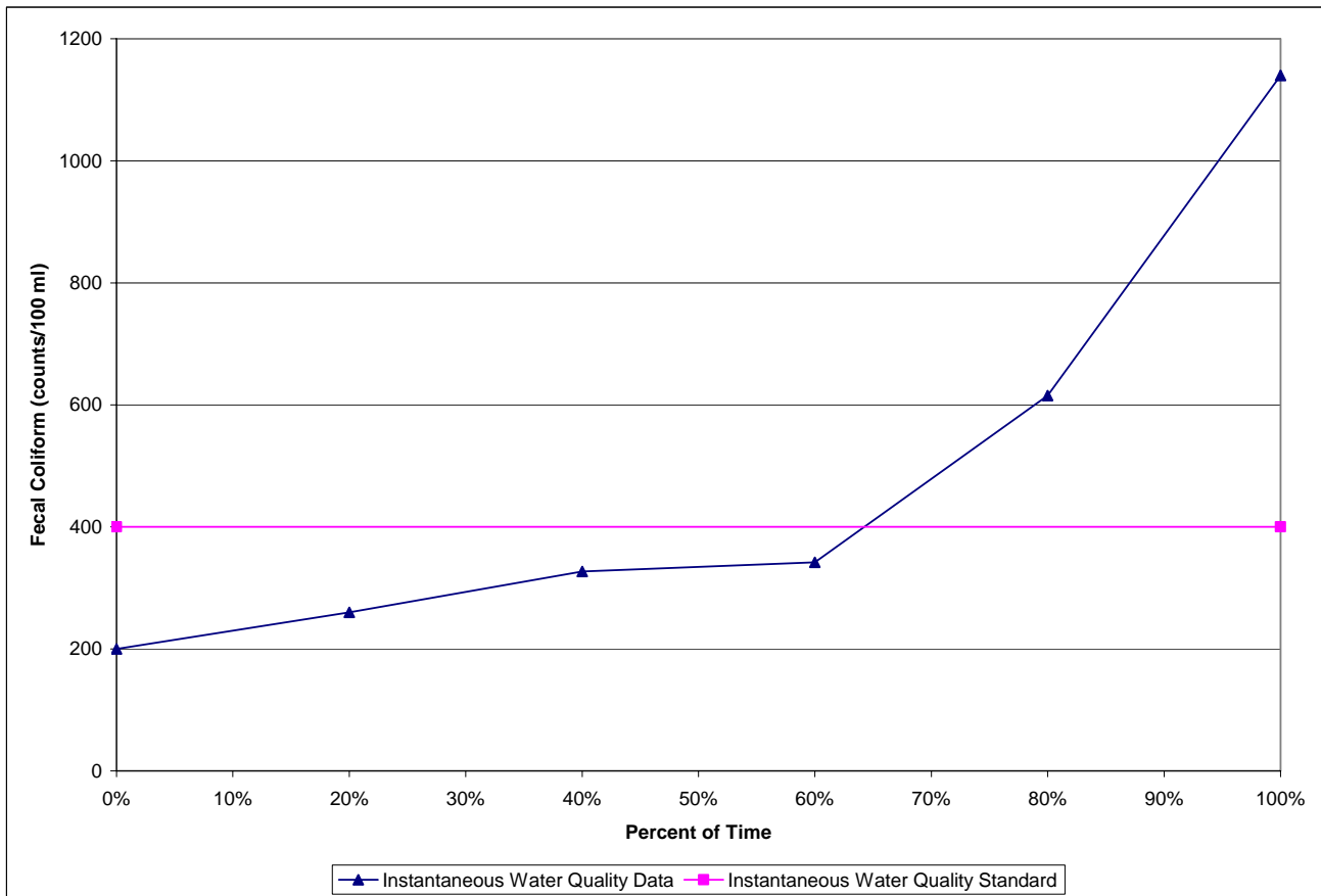
Figure 5. 10% Test Curve for Station A0630003, Summer 2006
